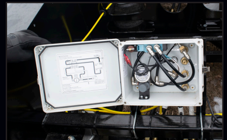
LIFT AXLE CONTROL VALVE ASSEMBLY
